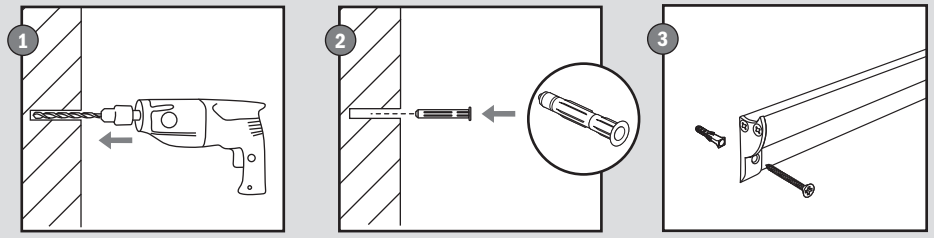
STAS paperrail > wall mounting
